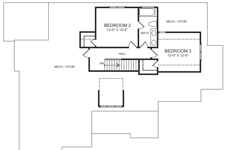
SECOND FLOOR
